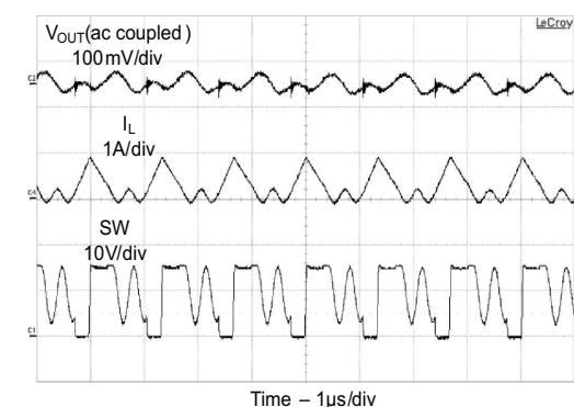
Figure 26. Output Ripple in DCM
