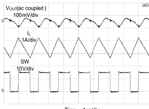
Figure 25. Output Ripple in CCM
